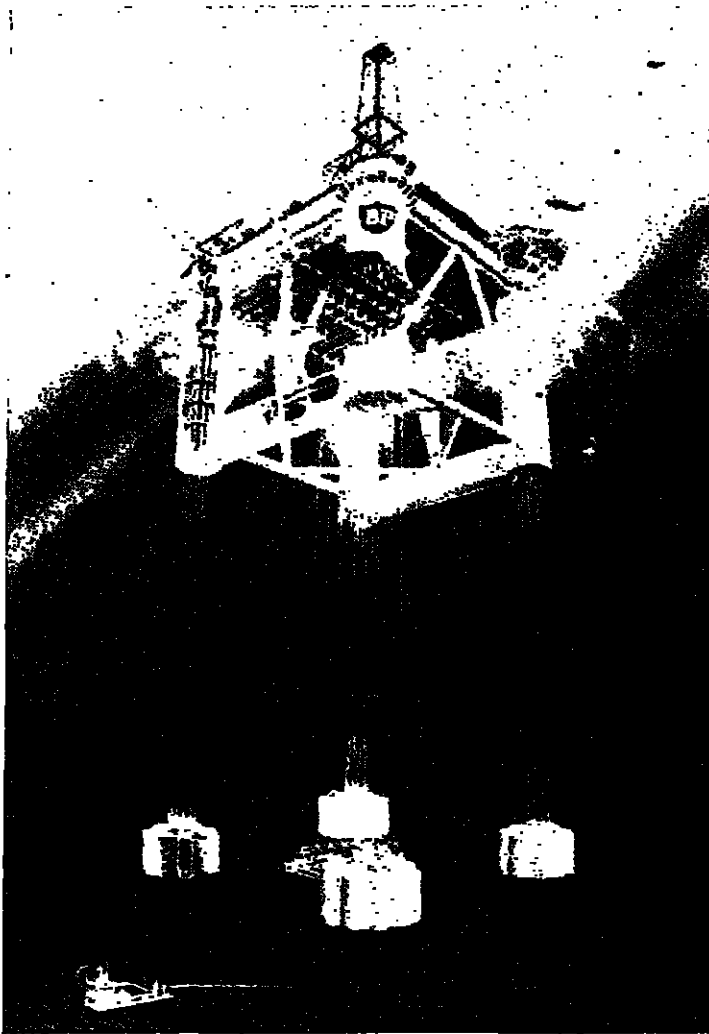
An artist's impression of the tension leg production platform, a new type of structure capable of drilling in water three times deeper than any platform of current design can operate in. It is designed to float, tethered by vertical mooring lines to seabed anchors that would hold it in enforced displacement at a predetermined level deeper than it would normally float. First probable use of the structure will be in the Hutton field in the North Sea, due to come on stream in 1984.
